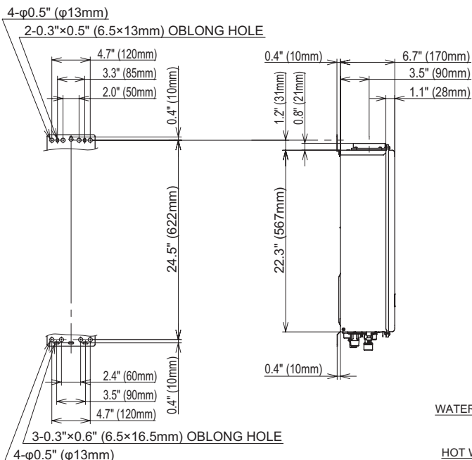
HEIGHT OF EACH FITTING FROM BOTTOM OF CASE
